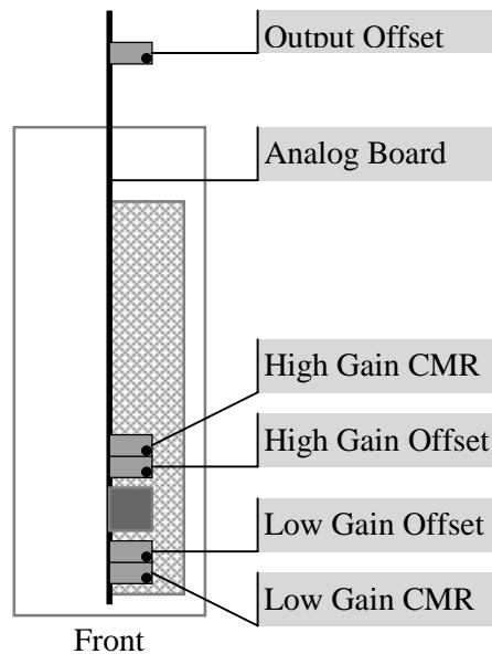
Figure 8-3 Analog Adjustments
